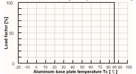
CFB750-300SXX Derating
